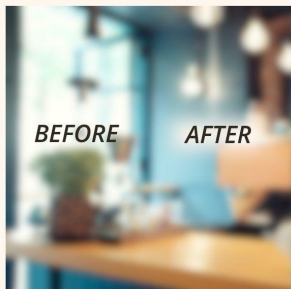
Blur object:
