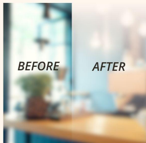
Overlay:
